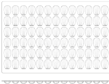
MID MADELAINE 78 Cups Cup Size: 46 x 33 x 15mm Capacity: 11ml Item No. 54830
