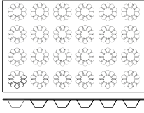
BRIOCHE 24 Cups Cup Size: 79 x 35mm Capacity: 84ml Item No. 54801
