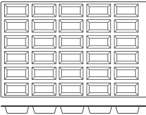
MINI CAKE 30 Cups Cup Size: 99 x 49 x 30mm Capacity: 110ml Item No. 54806
